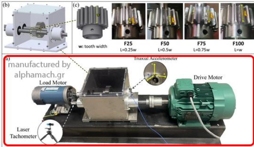
Figure 4. The experimental set-up: (a) photo of the gearbox including the sensors (accelerometer and tachometer) locations, (b) cross-sectional view of the one-stage gearbox and (c) the pinion single-tooth fault scenarios F25, F50, F75 and F100.
